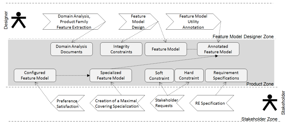
Figure 4. The overview of the interactive feature model configuration process.
