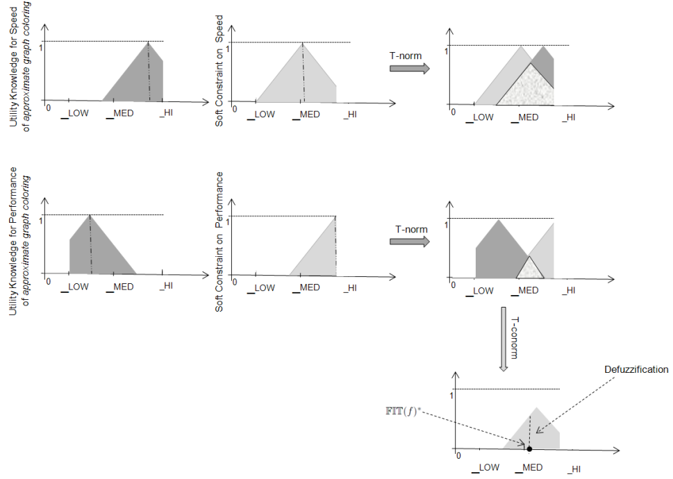
Figure 5. Computing the fitness of a feature f within the context of two concerns: speed and performance.
