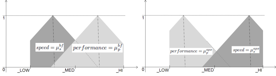
Figure 3. The Semantic annotation of a) brute force and b) approximation graph coloring features.
