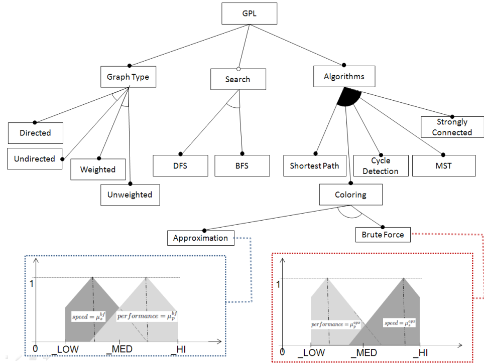
Figure 6. Annotate feature model with information regarding important domain concerns.
